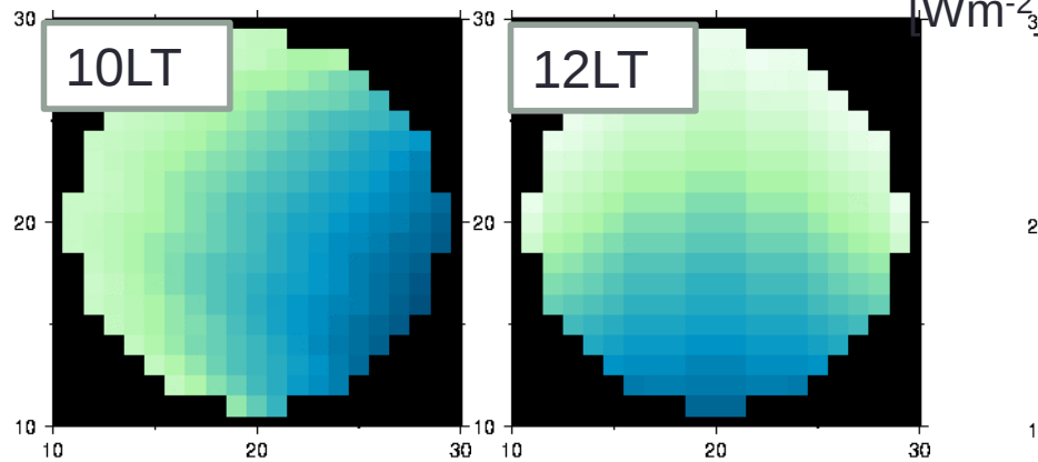
Sensible Heat
