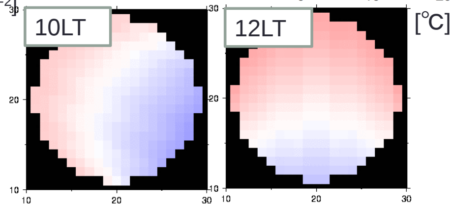
Latent Heat
