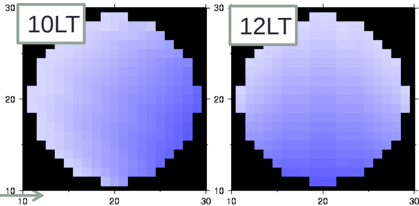
Sensible Heat
