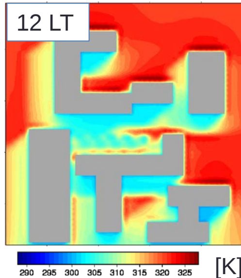
Surface Temperature
