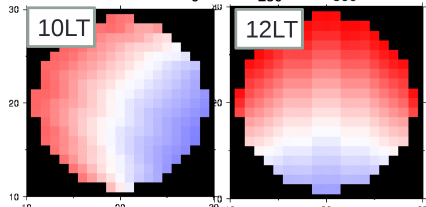
Latent Heat
