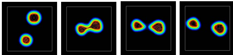
TDHF simulation to produce neutron-rich nuclei by multi-nucleon transfer reaction
