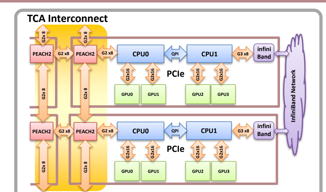
Block diagram of computation node of HA-PACS/TCA
