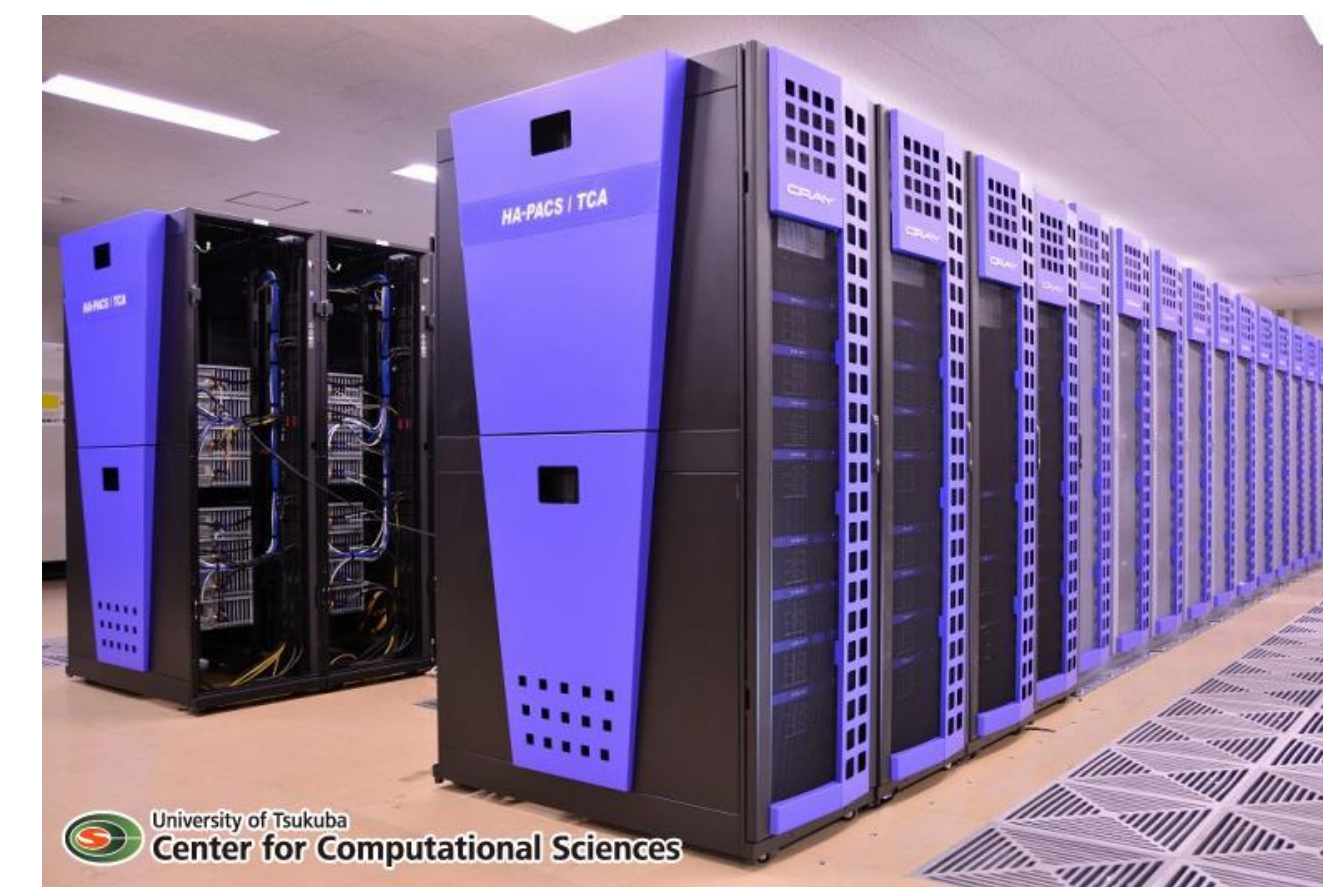
HA-PACS
